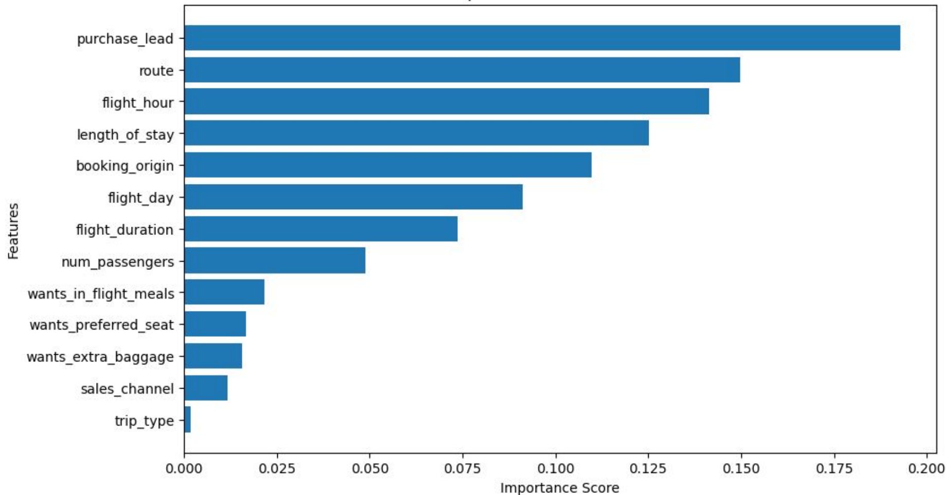
Feature Importance in Random Forest Model
